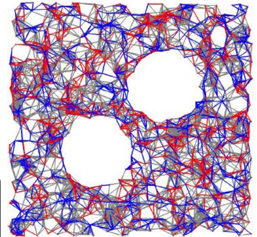
(a) The planarization constructed by ZJC-algorithm.
