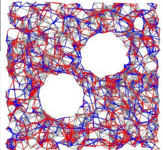
(b) The planarization constructed by our algorithm.
