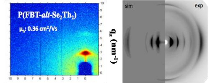
GI-XRD
