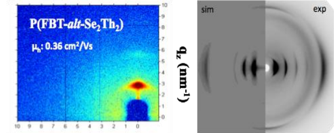
GI-XRD
